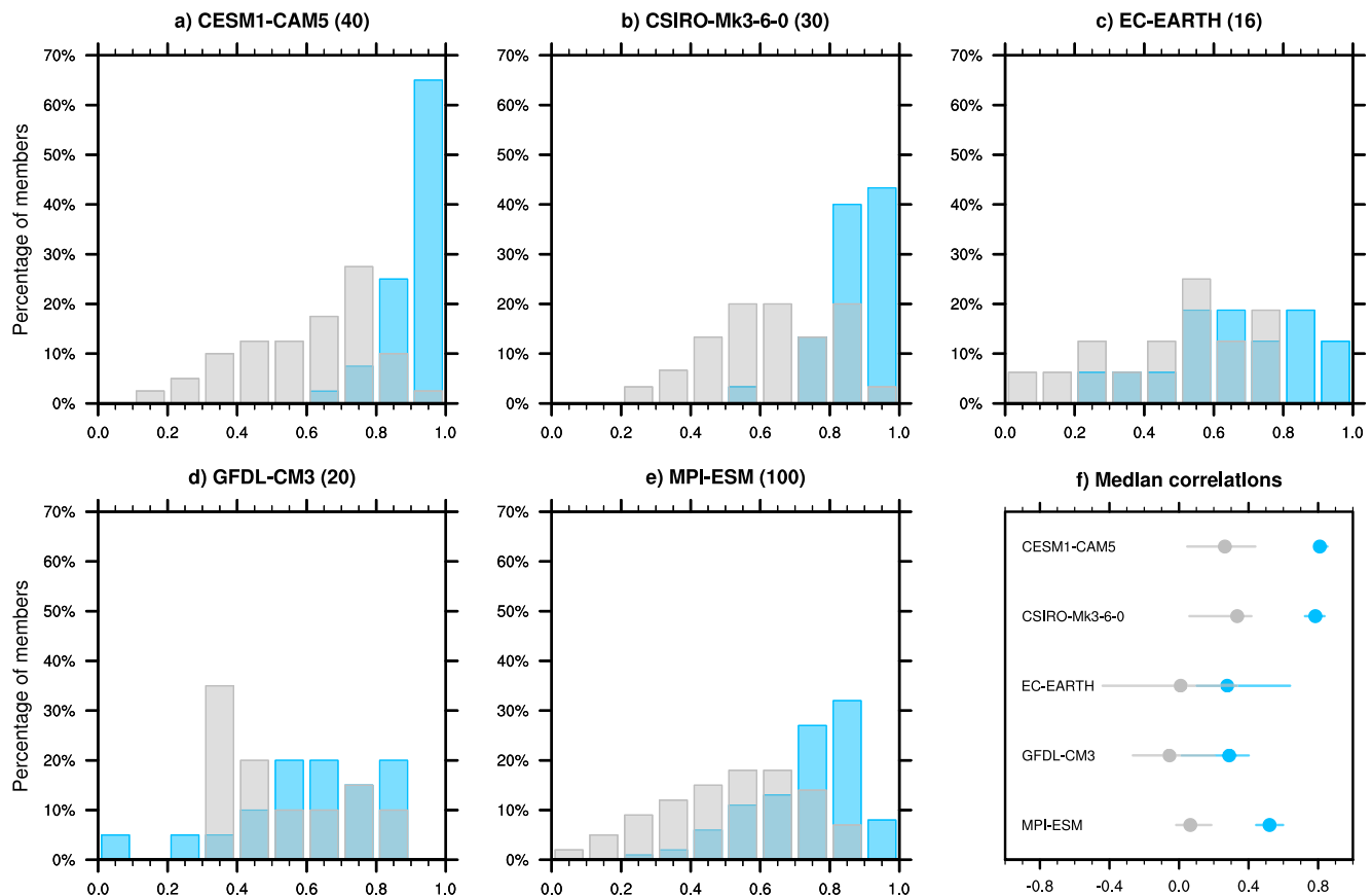
Figure 4. Histograms of correlation coefficients between Arctic and Antarctic multi-decadal surface temperature fluctuations in individual members of five of the LEs (a–e) for the period 1920-2019. The number of members in each LE is shown in parentheses. (f) An estimate of the median correlation value for each model with the 95% confidence interval. In each panel, the blue indicates the correlation of the anomalies from the linear trends and the gray instead indicates the correlations of the deviations from the ensemble mean.
